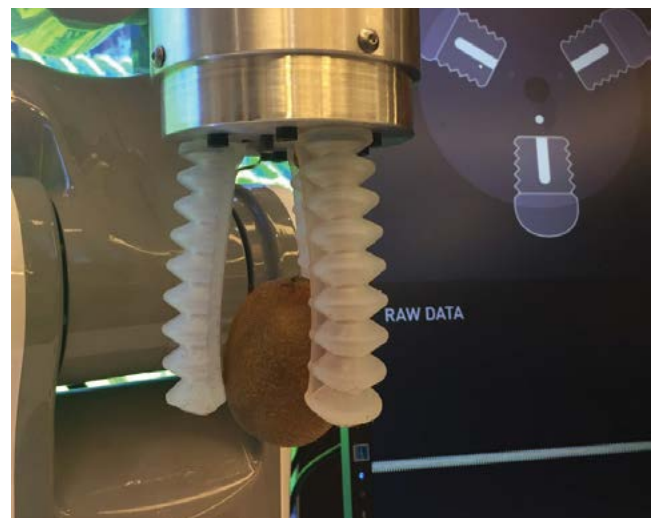
FIGURE 6: Slip sensors built into flexible end effectors enable minimum application of force for picking of fruit.
